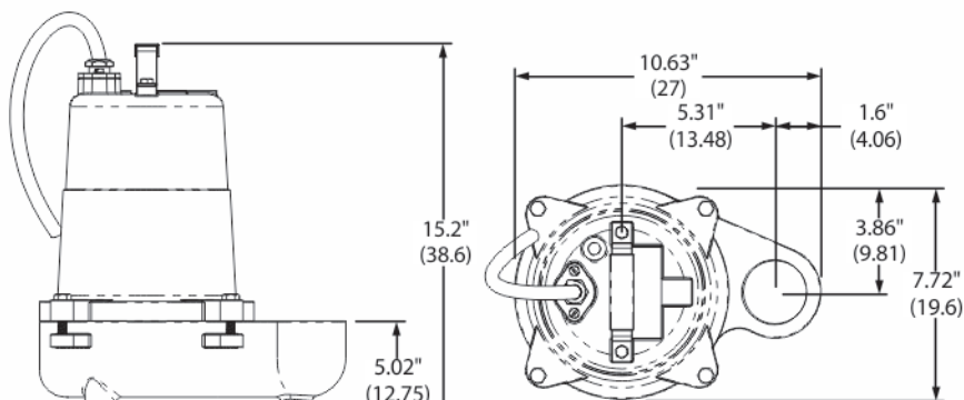
DIMENSIONAL
